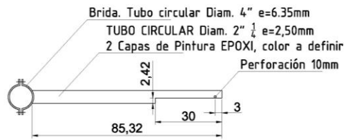
VISTA FRONTAL
